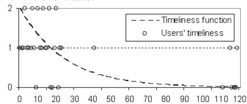
Figure 4: News:Timeliness functions vs users' evaluation.
