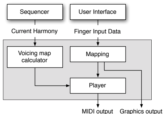
Figure 10 Voicing algorithm global structure
