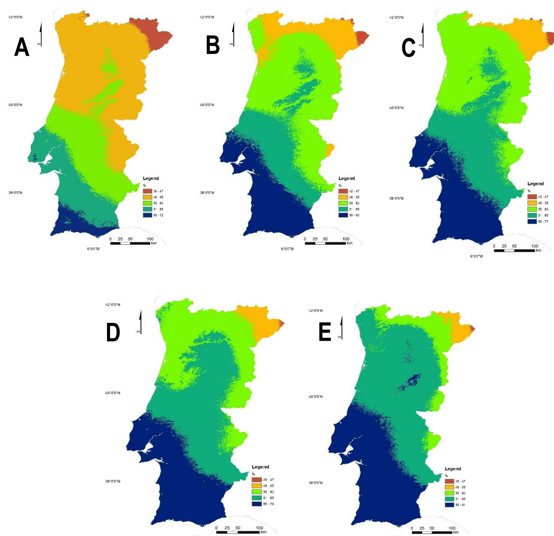
Fig 3. Representation of BIO15 variable, the precipitation seasonality in %, that has highest contribution for the A. unedo habitat suitability predictions in the Maxent. (A) Present (current climate conditions). (B) Future 2050, RCP 4.5. (C) Future 2070, RCP 4.5. (D) Future 2050, RCP 8.5. (E) Future 2070, RCP 8.5.
