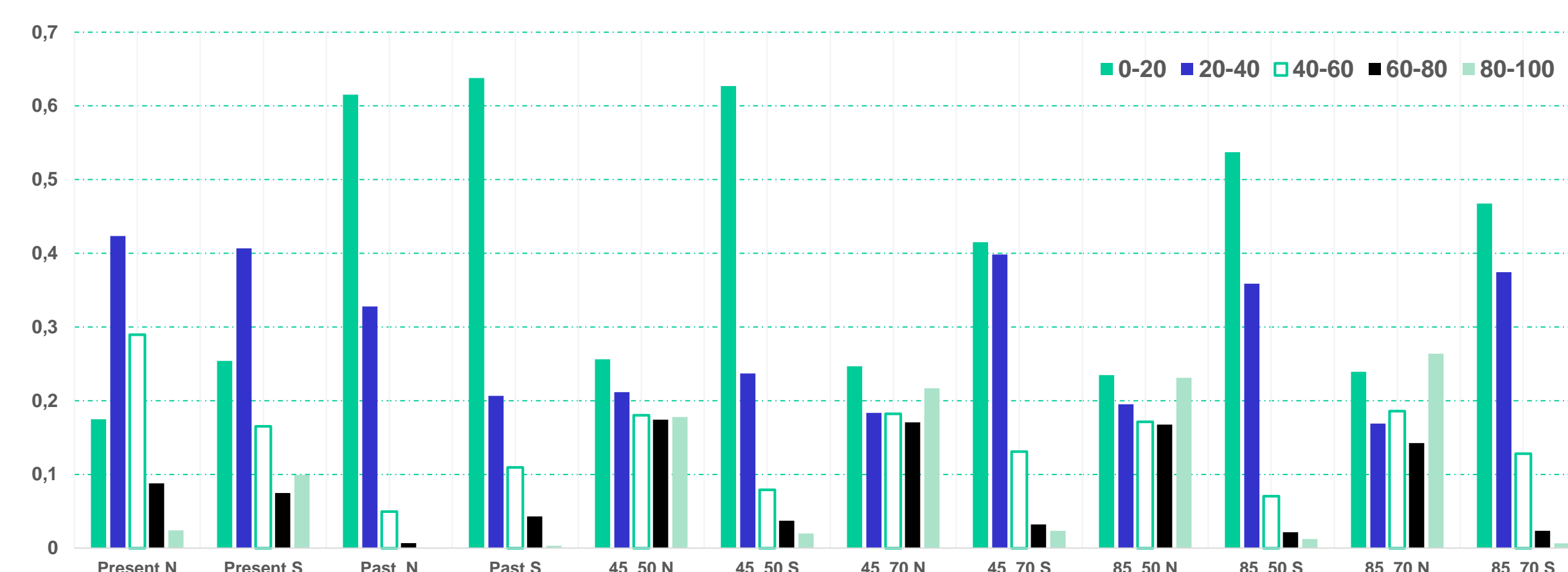
Fig. 4 Territorial evolution in percentage (area) of the present, past, future 2050 (RCP 4.5 and RCP 8.5), and future 2070 (RCP 4.5 and RCP 8.5) climate conditions, for the different classes of probability of presence of the species predicted conditions, in the North (N) and in the South (S) of the Tagus river.
