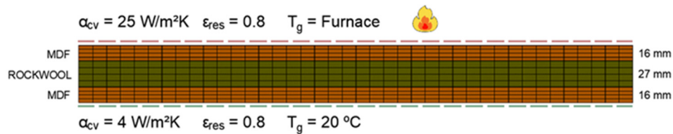
Figure 3: Boundary conditions of the finite element model.
