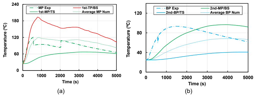
Figure 8. Thermal Outputs for Wood Pallet in (a) MP and (b) BP.
