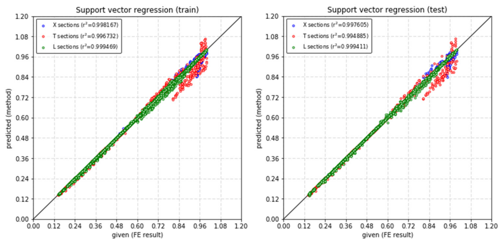
Figure 3 – Accuracy between obtained FE results and predicted by the support vector regression model for the training (left) and testing (right) sets.
