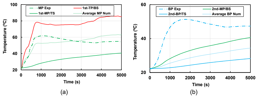
Figure 11. Thermal Outputs for Pine in (a) MP and (b) BP.
