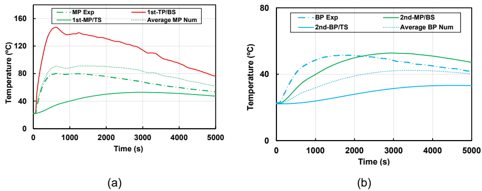
Figure 10. Thermal Outputs for Eucalyptus in (a) MP and (b) BP.
