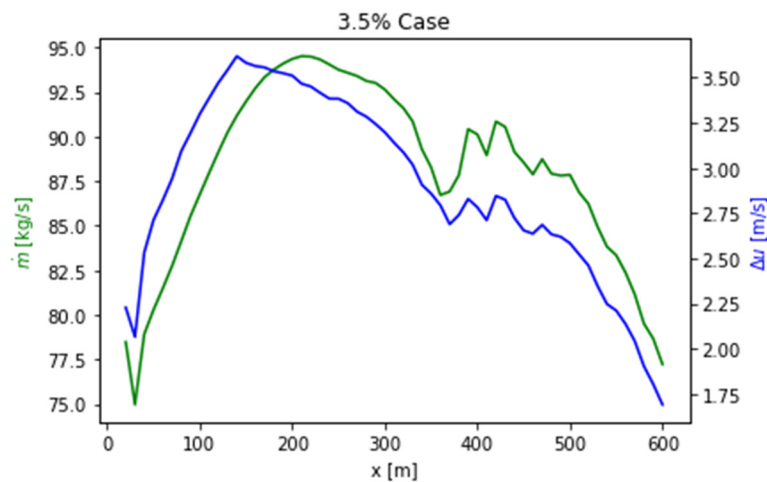
Figure 7: Mass flow rate at the upper layer and difference between the average velocity at the upper and lower layers
