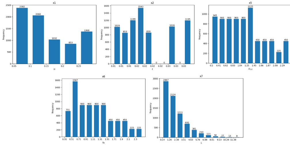
Figure 1: Example frequency distribution for some input features considered for the L-shape cases.
