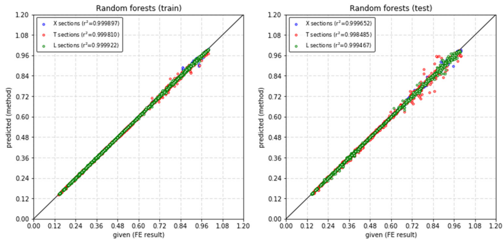
Figure 4 – Accuracy between obtained FE results and predicted by the random forests model for the training (left) and testing (right) sets.
