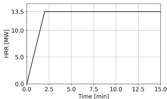
Figure 3: Heat release rate curve
