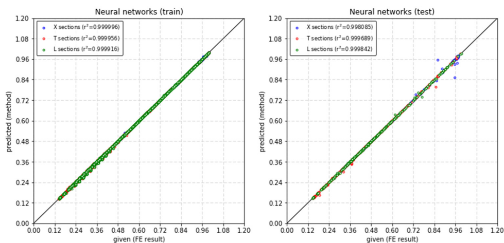
Figure 2 – Accuracy between obtained FE results and predicted by the neural network model for the training (left) and testing (right) sets.
