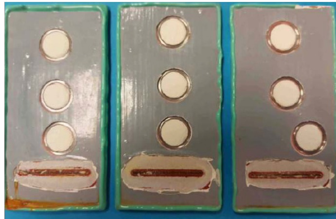
Image 2: small panels after salt spray testing and removal of the coating around the scribe to evaluate corrosion advance
