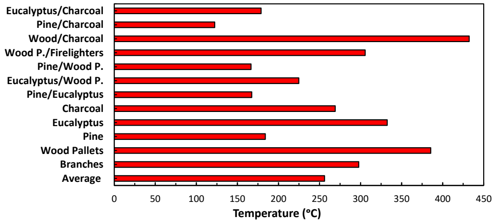
Figure 3. Maximum temperatures for the specimens.
