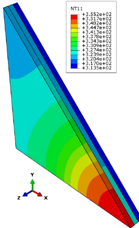
Figure 7. Temperature field distribution for Wood Pallets for 6000 s (temperature in Kelvin).
