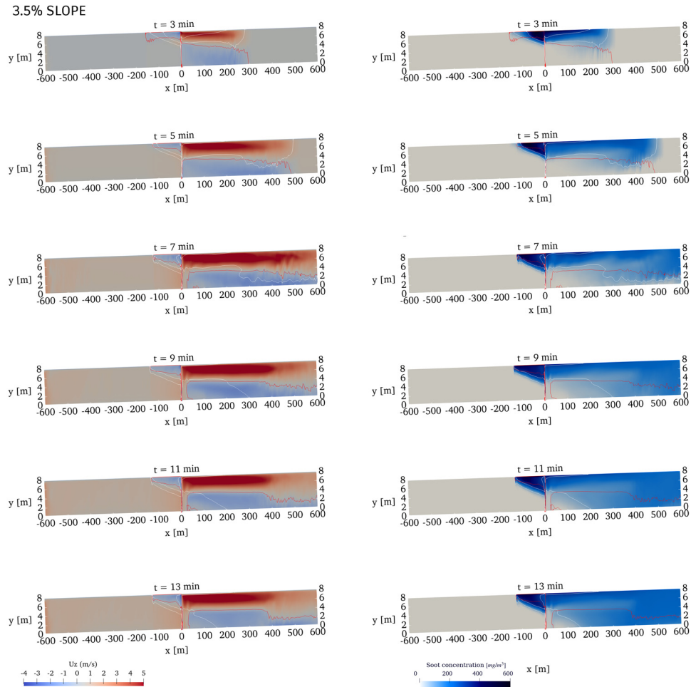
Figure 4: Soot and velocity fields for a tunnel with a slope of 3.5%.
