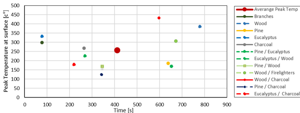
Figure 5 – Maximum peak temperatures for the different type of woods.
