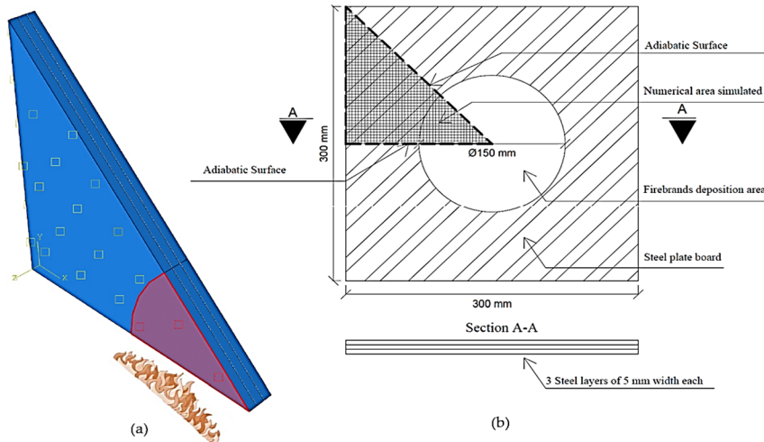
Figure 4. Geometry used in which (a) is the numerical model and (b) experimental schematic setup.
