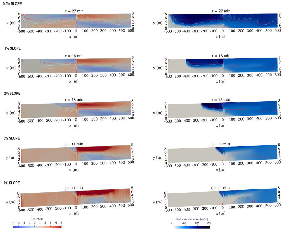
Figure 5: Steady state fields of velocity and soot concentration for simulations A (0.5%) to F (7.0%)
