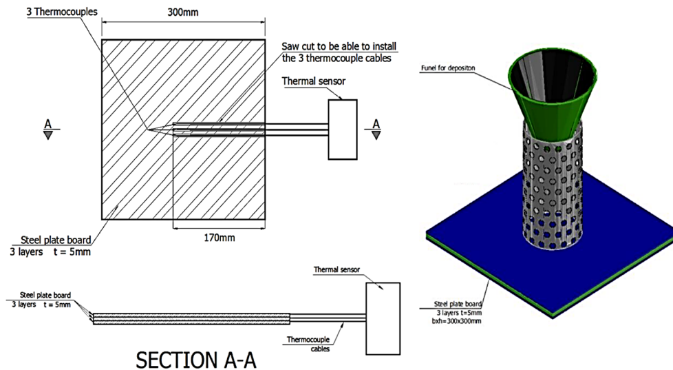
Figure 2. Experimental set-up [43].
