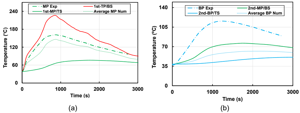
Figure 9. Thermal Outputs for Wood-Charcoal in (a) MP, (b) BP.
