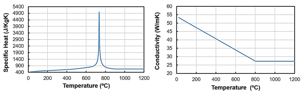
Figure 5. Specific Heat and Thermal Conductivity used [47].
