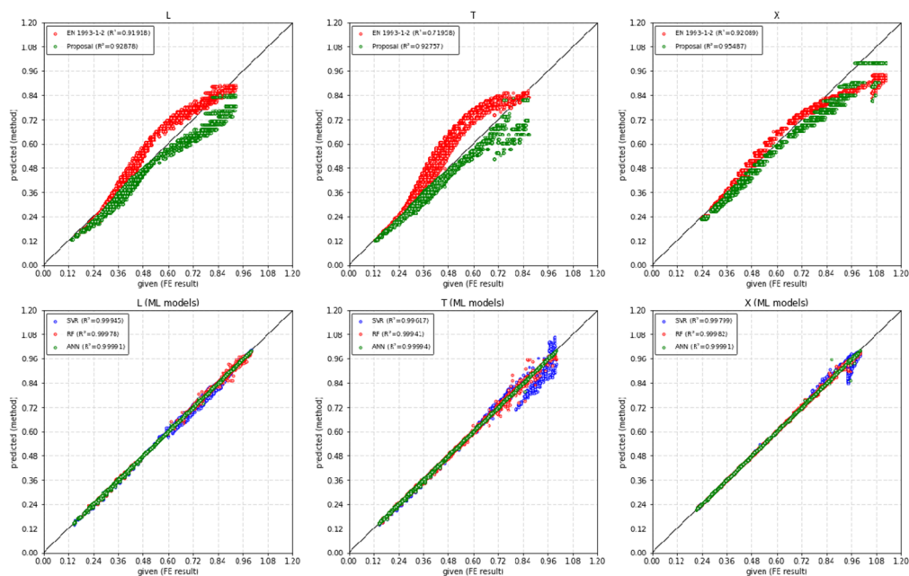
Figure 5 – Comparison between obtained FE results and predicted by the analytical methods (top) and with the ANN, RF and SVR machine learning models (bottom).
