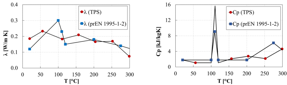
Figure 1: Thermal conductivity and specific heat of MDF at temperatures up to 300 °C.
