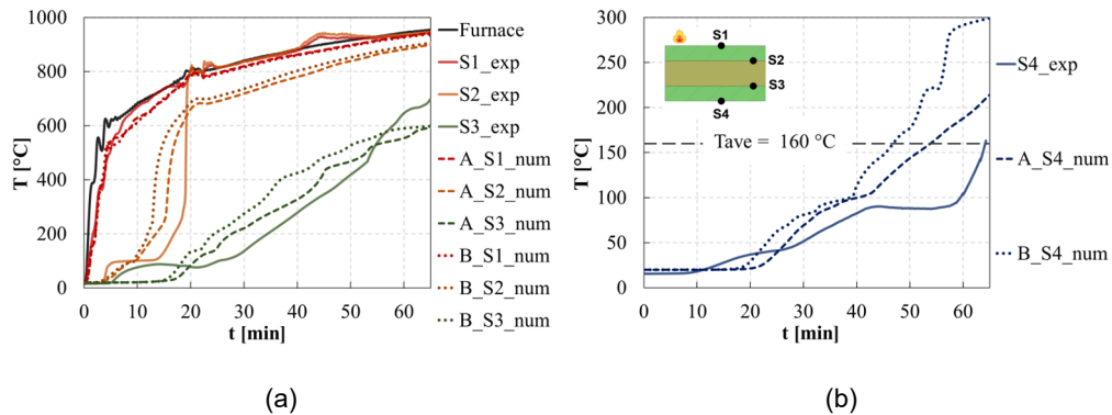
Figure 4: Comparison between the temperature history obtained in the experimental test (exp) and finite element simulations A and B (num).
