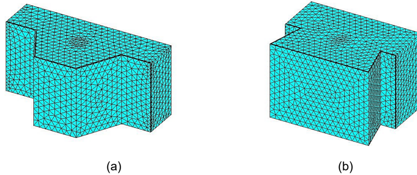
Figure 5: Finite elements mesh: (a) Trapzoidal and (b) Re-entrant profile.
