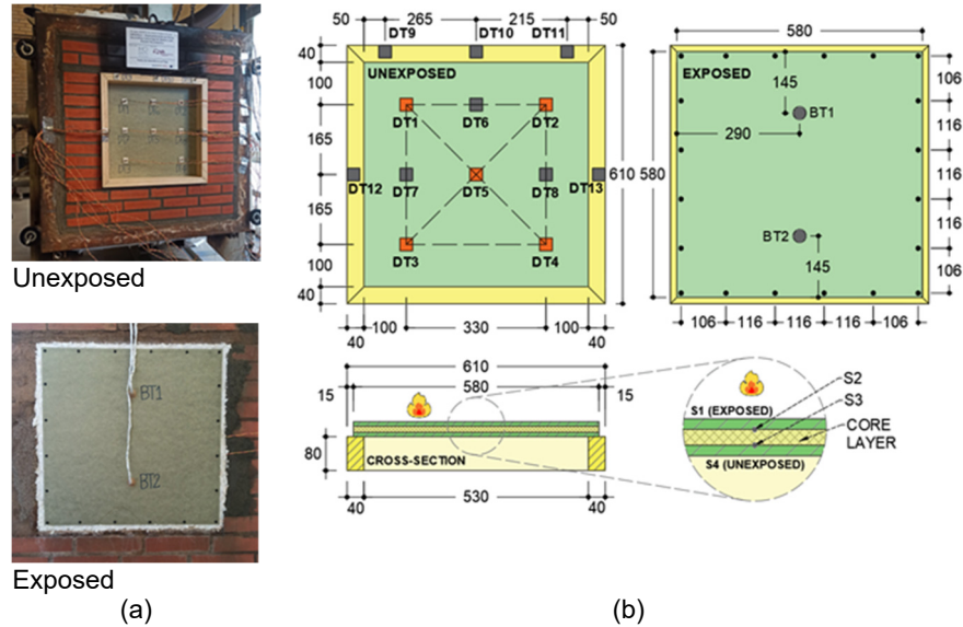
Figure 2: (a) View from the unexposed and exposed side of the experimental test and (b) Location of the thermocouples at different positions. Measurements in [mm].
