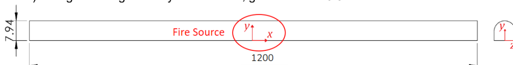
Figure 1: Dimensions [m] of the tunnel and reference frame centred at the fire source. The width of the tunnel is 8.56 m.
