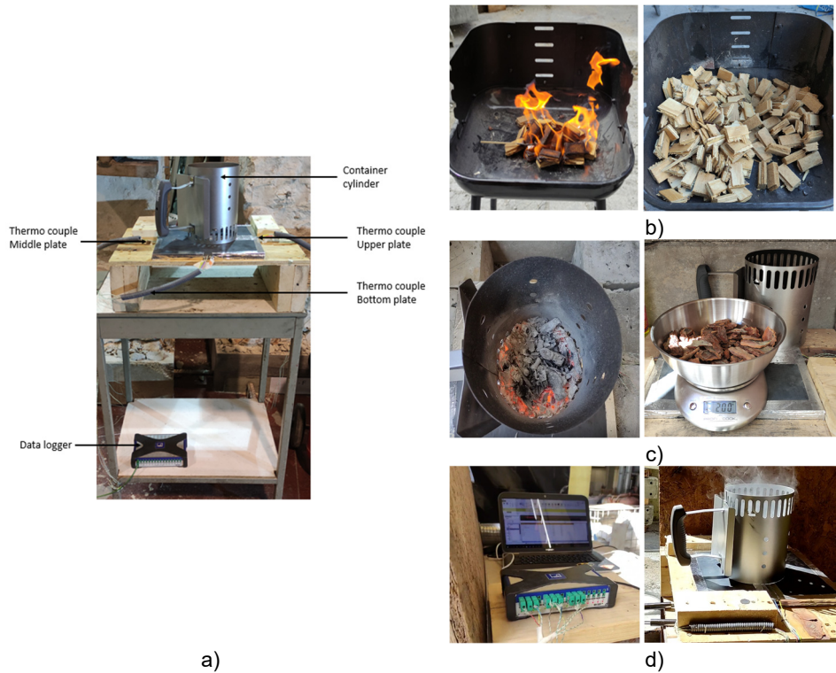
Figure 3 – Laboratory setup procedure (a) full laboratory setup, (b) wood sample and wood burning (c) 200g wood sample and weight of burned firebrands, (d) plates with thermocouples and recording data.
