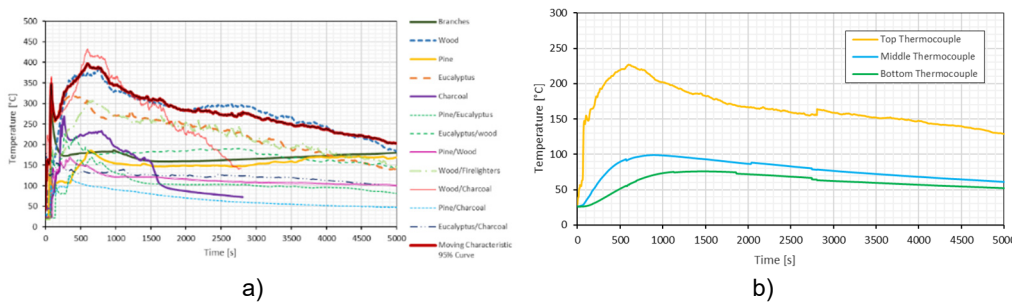
Figure 4 – Thermocouples temperature output: a) Top thermocouple; b) Average temperatures of all specimens for the top, middle and bottom thermocouple.
