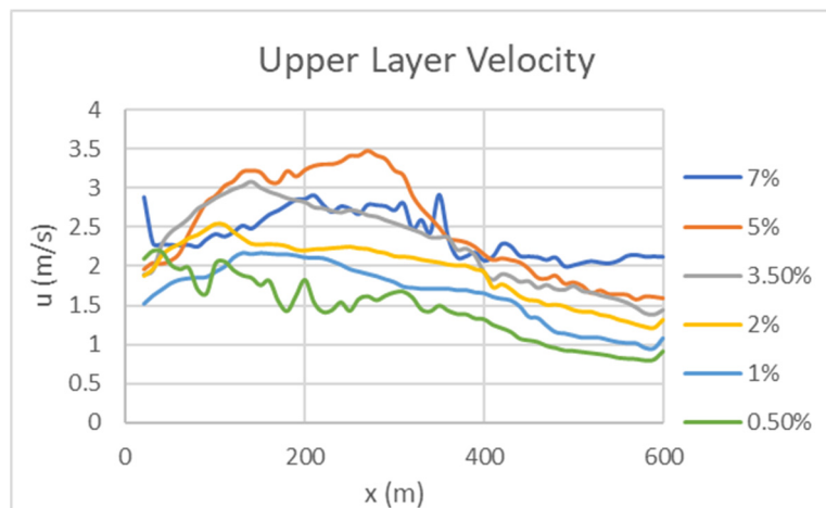
Figure 6: Average upper layer velocity from the fire to the upper portal for simulations A to F
