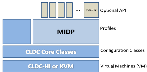
Figure 1 - Software architecture.
