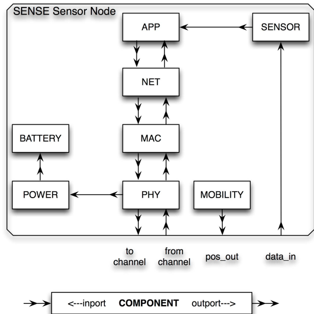
Figure 1. The internal structure of a typical sensor node model for WSNs in SENSE [5].
