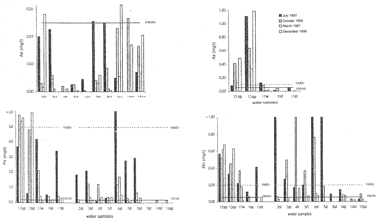
Figure 2 Seasonal variations for As, Fe and Mn water contents from the Segura area
